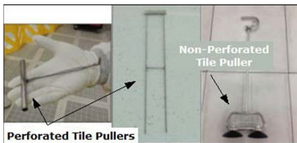
Figure 18 Tile Pullers
