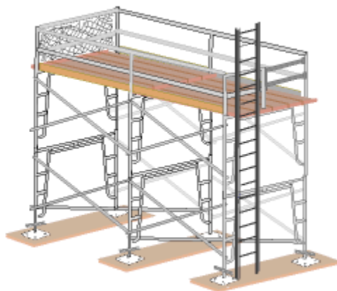
Figure 28 Frame Scaffold
