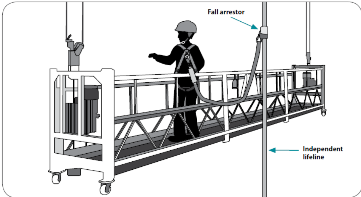
Figure 30 Suspended Scaffold
