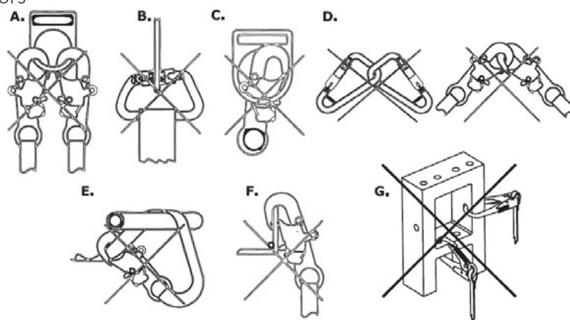
Figure 11 Connectors
