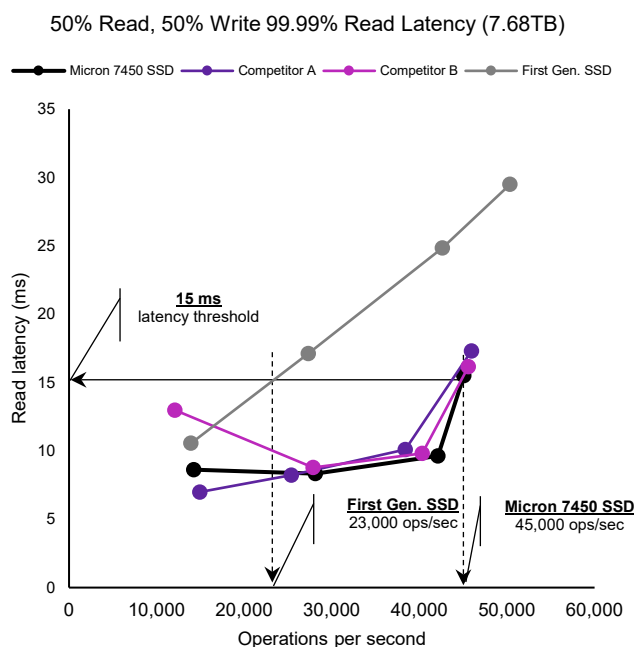
Figure 3: 99.99% latency vs. operations per second – 15 milliseconds
